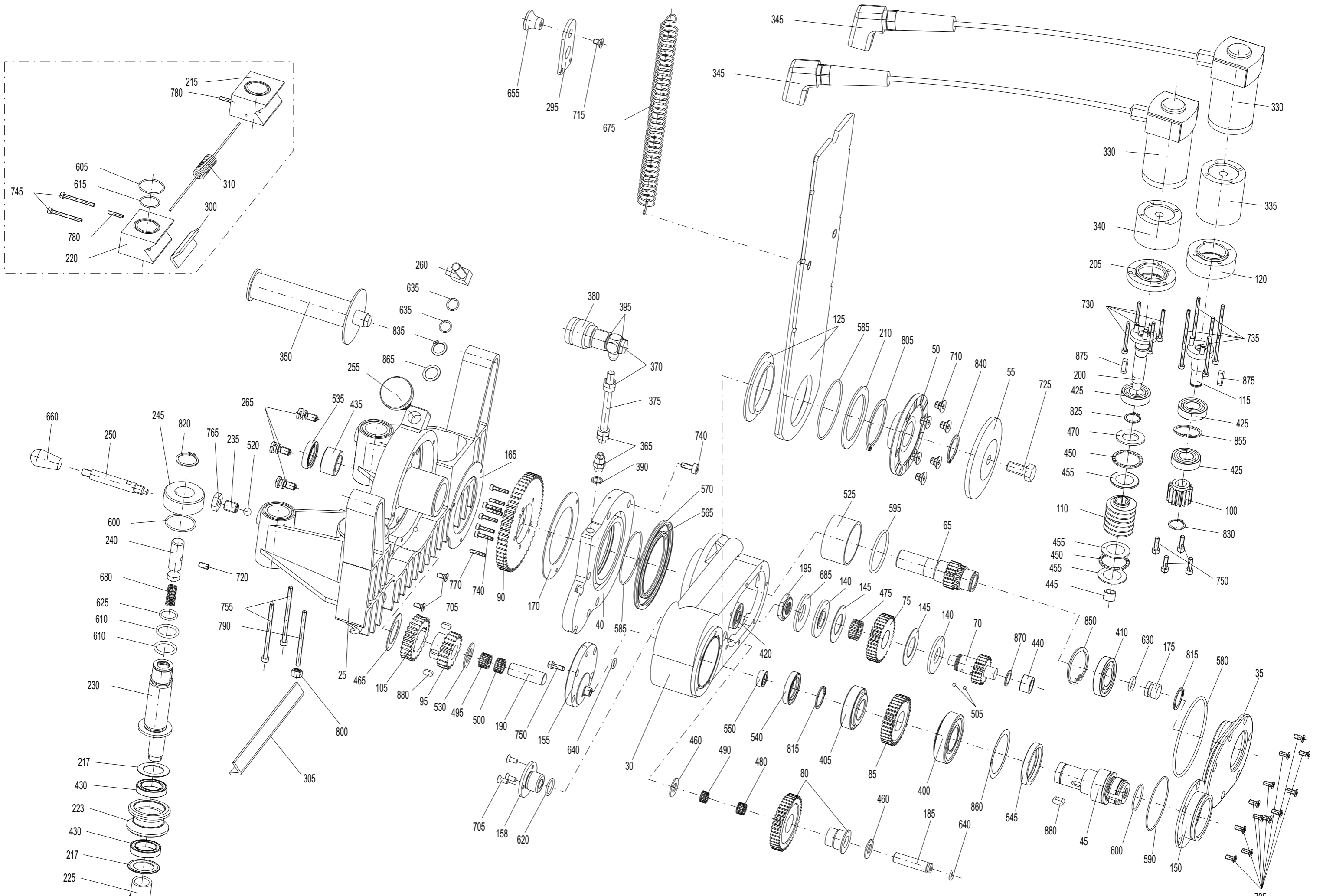
Diamond Wall Saw WS 75 H Carriage WS 8020
